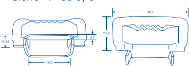
Cierre "T" SS 5/8"
