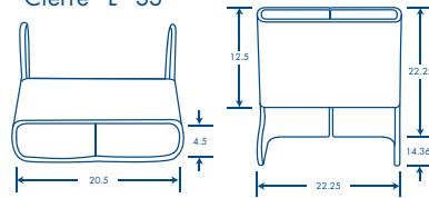
Cierre "L" SS
